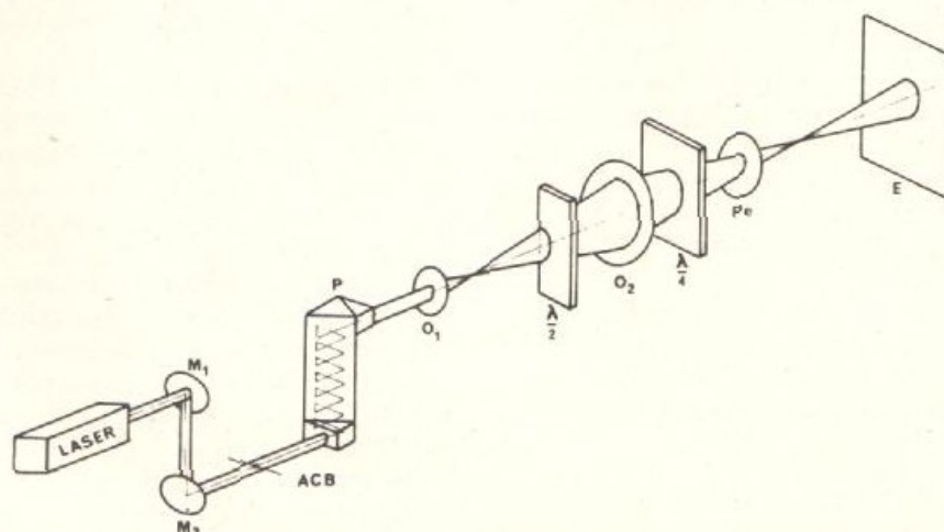
FIG. 6. The over-all experimental arrangement: unpolarized laser, rectilinear object, multiplying prism where the beam undergoes 28 near-to-limit total reflections, half-wave plate covering half of the beam, circular polarization analyzer (quarter-wave plate and linear polarizer), amplifying lenses, and screen receiving the image of the rectilinear object.
