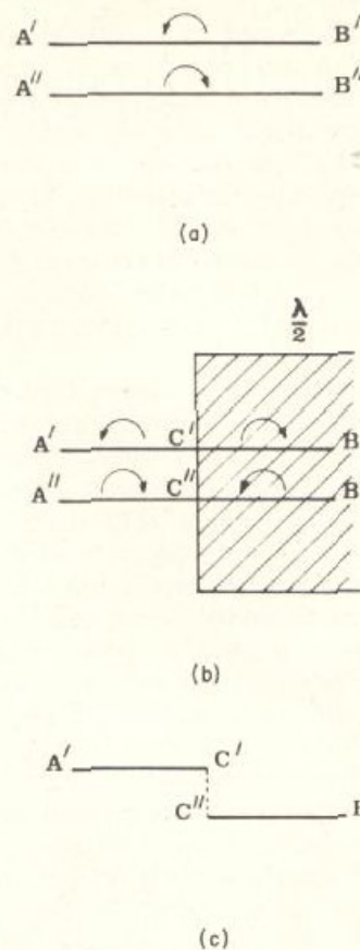
FIG. 5. The "trick" for unraveling the two overlapping circularly polarized eigenfunctions (a) of the transverse shift: (b) a half-wave plate covering half of the beam reverses the circular polarizations; then (c) a circular polarization analyzer suppresses one of the two states.
