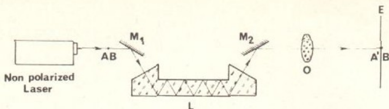
FIG. 3. Our version of the Goos-Hänchen-type device for amplifying the longitudinal shift in total reflection.
