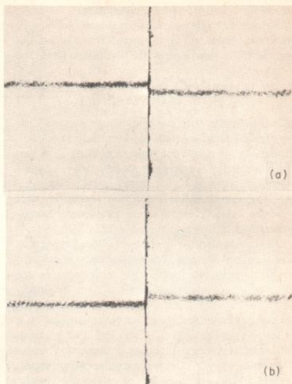
FIG. 7. The two symmetric broken images of the rectilinear object displaying the two eigenvalues and the two eigenfunctions (circular polarization states) of the transverse shift. (a) left circular polarization suppressed; (b) right circular polarization suppressed.
