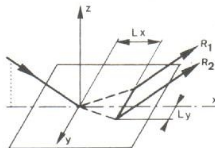
FIG. 2. Schematic representation of the longitudinal and the transverse shifts (in fact they are not simultaneously observable, as their eigenmodes belong to two different orthogonal sets).
