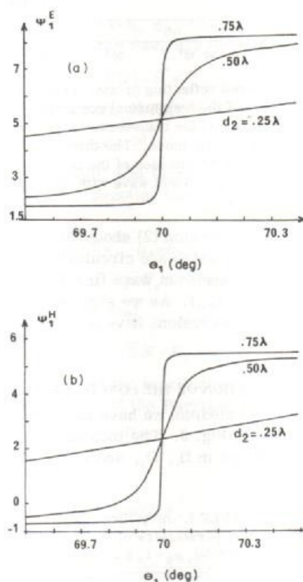
FIG. 6. 4-layered reflecting prism: This figure shows the incidence-angle dependence of the phase shifts between the incident and the reflected waves for (a) the transverse electric and (b) the transverse magnetic modes. The three curves correspond to three different thicknesses of the layer \Omega_2 . The phases are referred to one of the evanescent waves. Notice that the curves are slightly nonsymmetrical.
