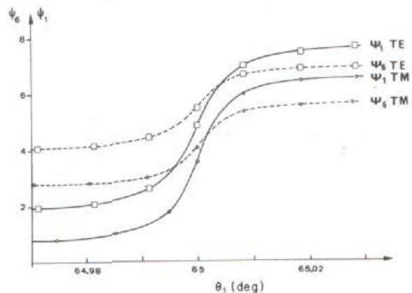
FIG. 9. 6-layered reflecting prism: This figure shows the incidence-angle dependence of the phase shifts \psi_1 of the reflected wave and \psi_e of the (final) evanescent wave.
