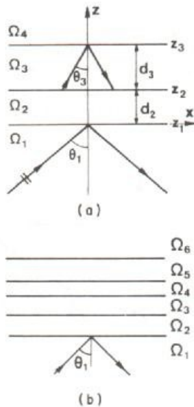
FIG. 3. Multilayered reflecting device for amplifying (a) the longitudinal and (b) the transverse energy flux; the wave propagating inside a layer is either of the homogeneous (sine and cosine), or of the inhomogeneous (sinh and cosh) type.
