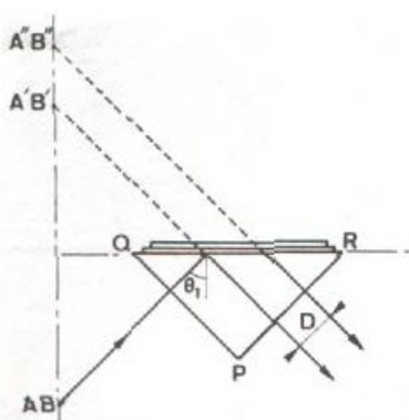
FIG. 12. Tunneling and nontunneling photons and the longitudinally shifted, and the nonshifted, reflected rays.
