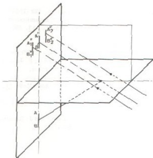
FIG. 17. Tunneling and nontunneling photons for the two transversally shifted A''B'' , A''B'' and the nonshifted A'B' images; AB is a linear object inside the incidence plane.
