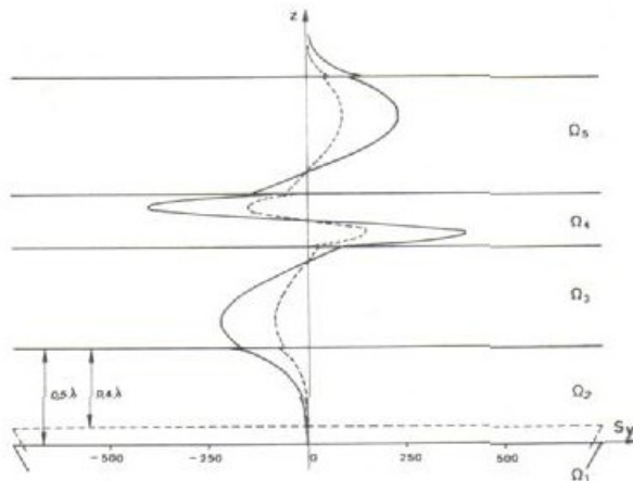
FIG. 10. 6-layered reflecting prism: z dependence of the transverse component S_y of the Poynting vector for two different thicknesses of the layer \Omega_2 . These are calculated curves corresponding to the ideal case where resonance occurs at the same angle for the TE and the TM modes.
