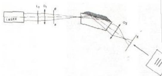
FIG. 18. Overall experimental setup for producing and observing the transverse shift, where L_1 is an orientable linear polarizer and AB is a linear object side the incidence plane.
